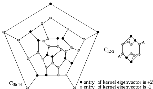
Figure 7: C_{36} : 14 and C_{12} : 2
