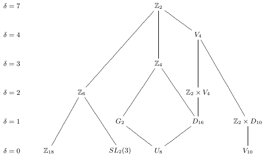
Figure 1: The lattice of automorphism groups for g = 4 .
