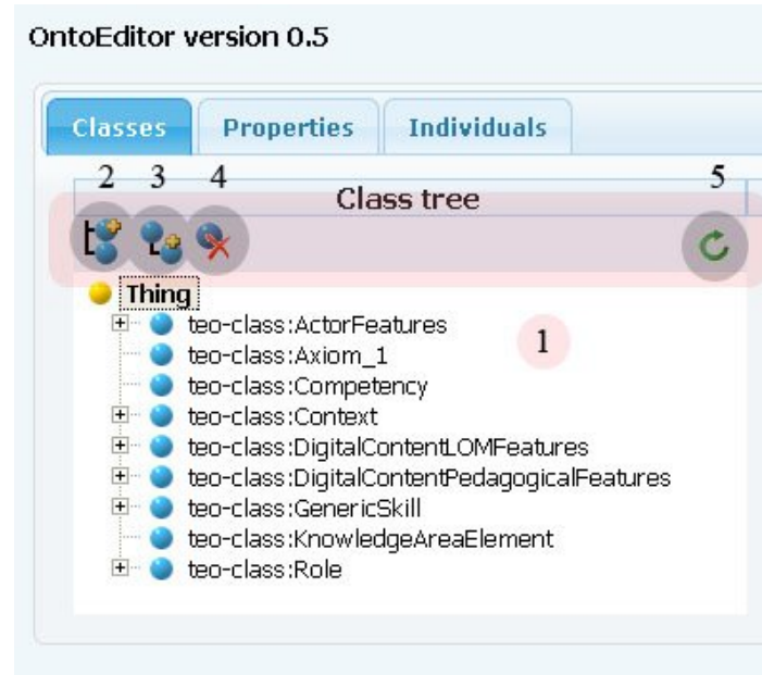
Fig.3. User interface of OntoEditor
