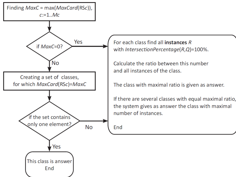
Figure 179. MPGN - Analyzing resulting recognition sets and making decision which class to be given as answer
