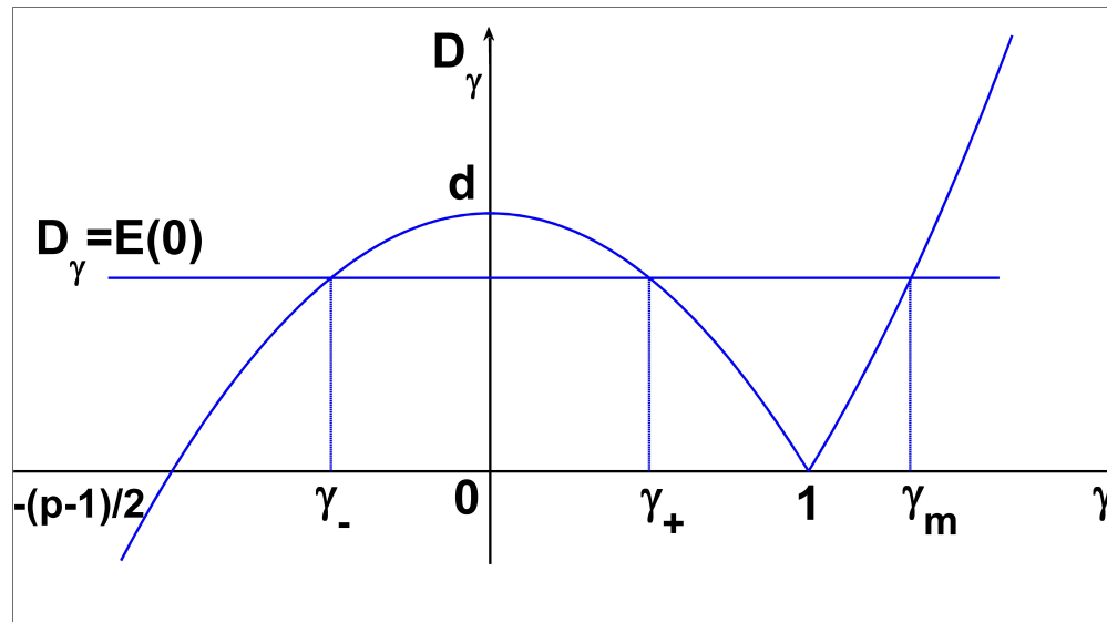
Figure 3: The graphics of D_\gamma as a function of \gamma for n = 1, p = 3 .
