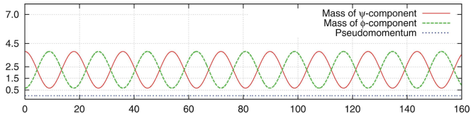
Figure: 14. \delta_l = 0^\circ , \delta_r = 90^\circ , P = 10^{-3} \div 10^{-5}
